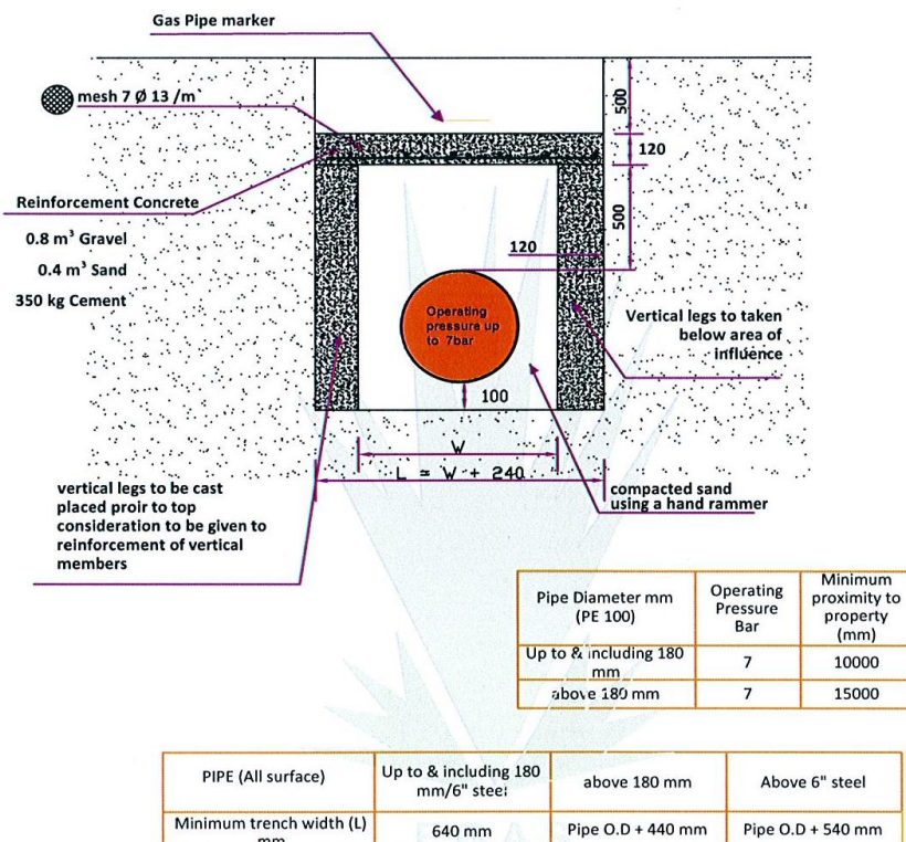
Figure 2-5: Typical layout of U-shaped concrete slab (Source: EGAS technical drawings)
