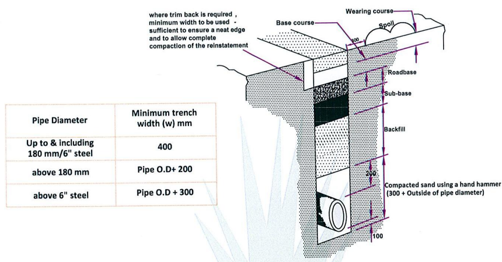
Figure 2-4: Typical backfill arrangement
