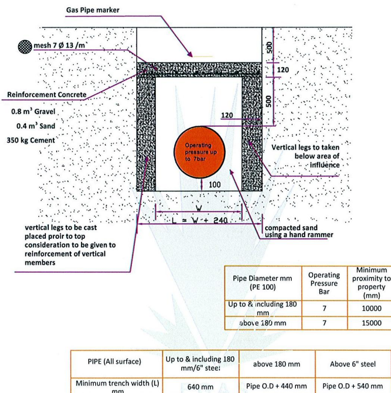
Figure 2-5: Typical layout of U-shaped concrete slab
