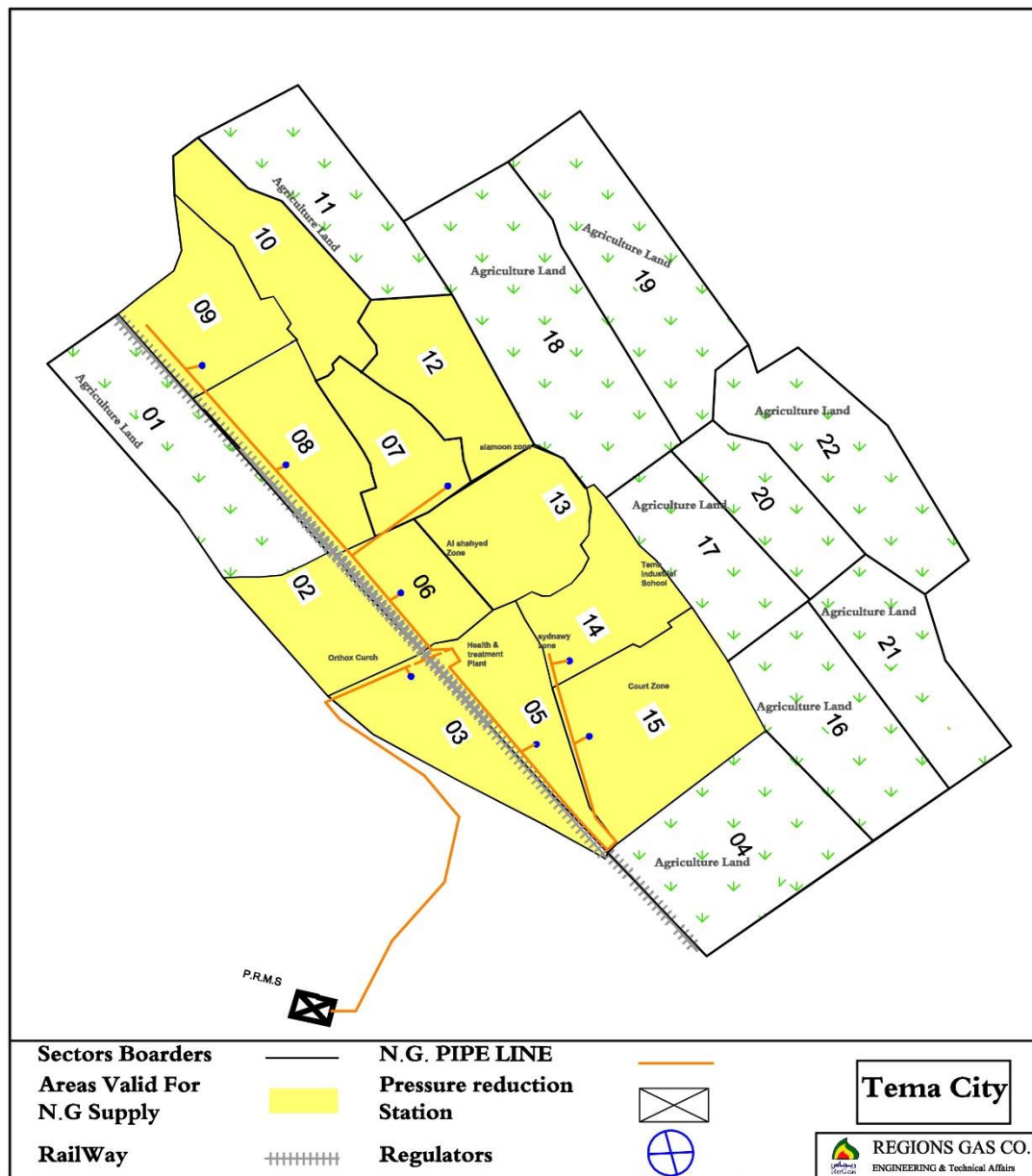
Figure 2-2: project sectors in Tema city
