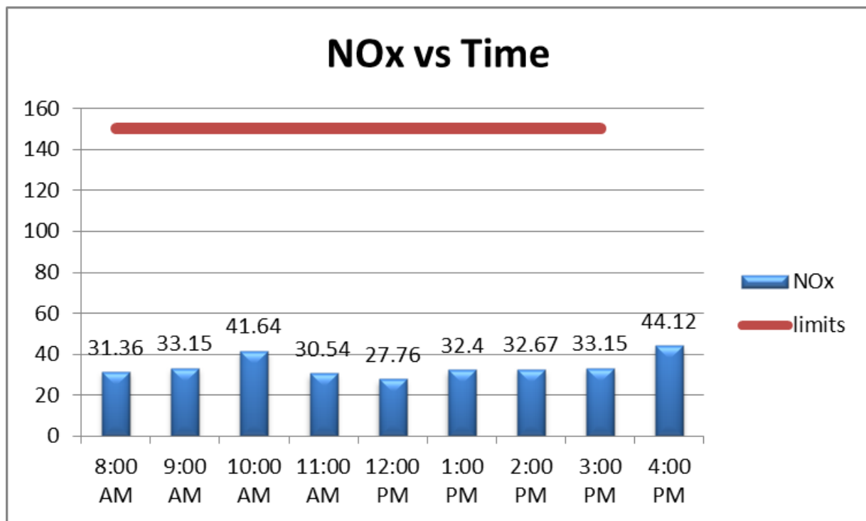
Figure 4-1 NO x variation in Hawamdyia
