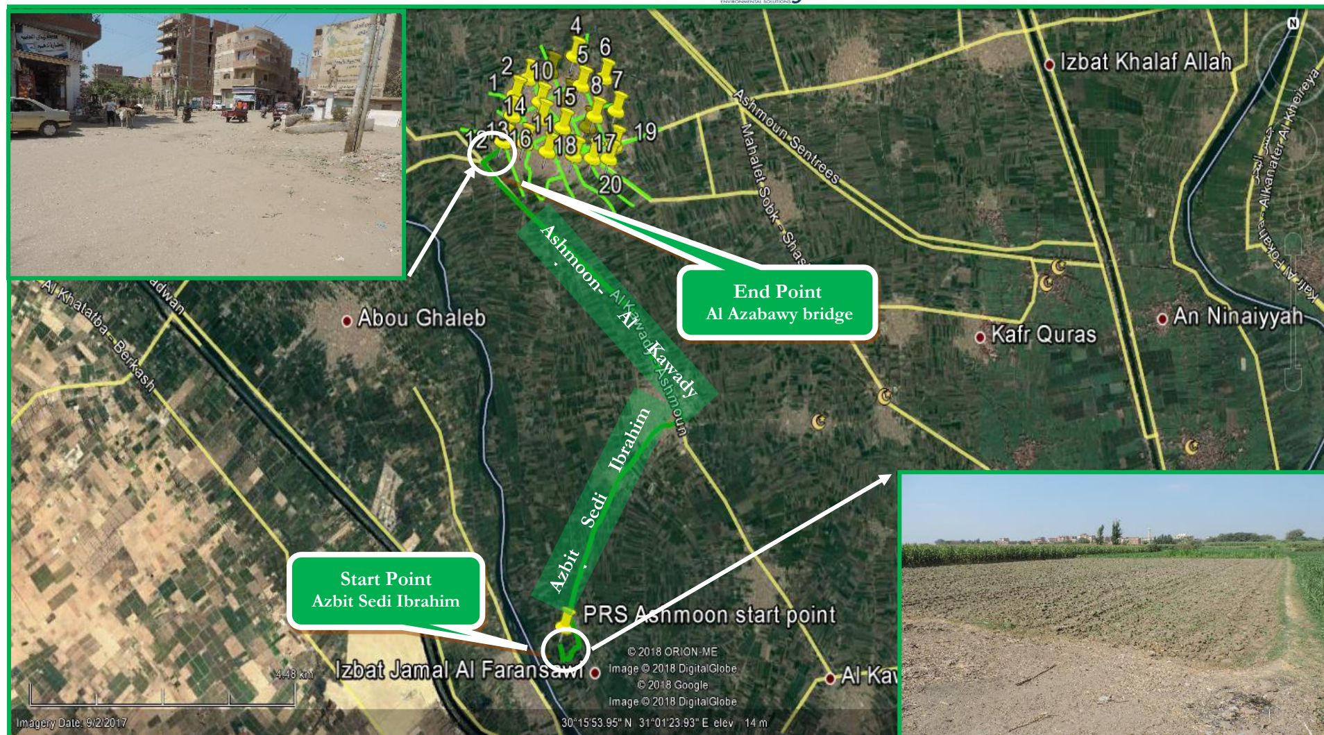
Figure 2-2: The proposed Ashmoon pipeline Network routes.
