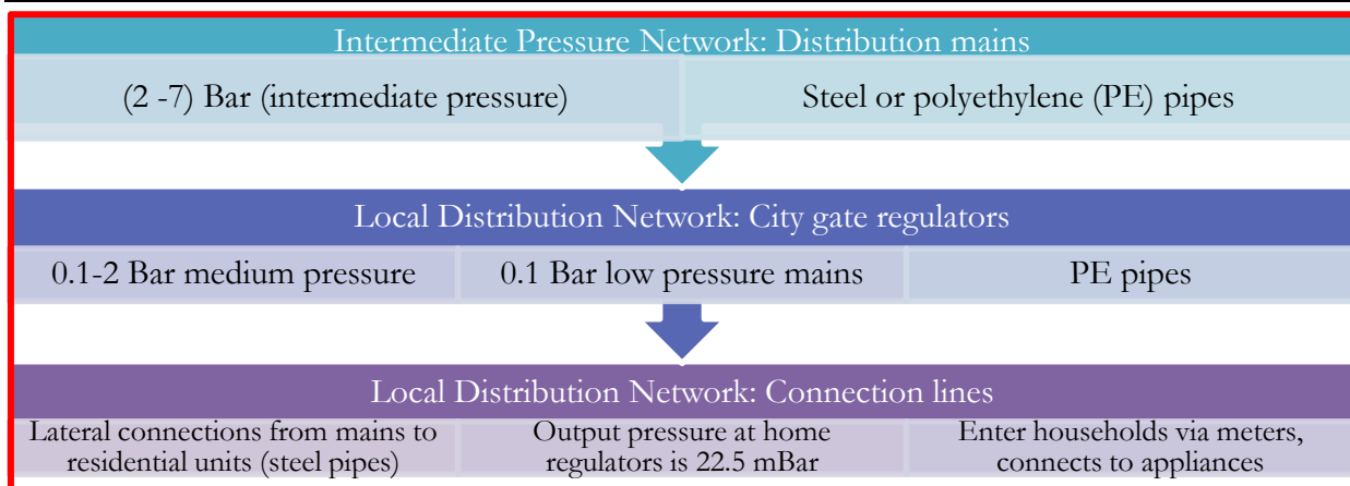
Figure 2-1: General components of the Shoubra Bakhom (Qwesna), Alshouhada, El Qum El Akhdar/El Batanoon, Ganzor and Ashmoon districts distribution network (Surrounded by red frame)
